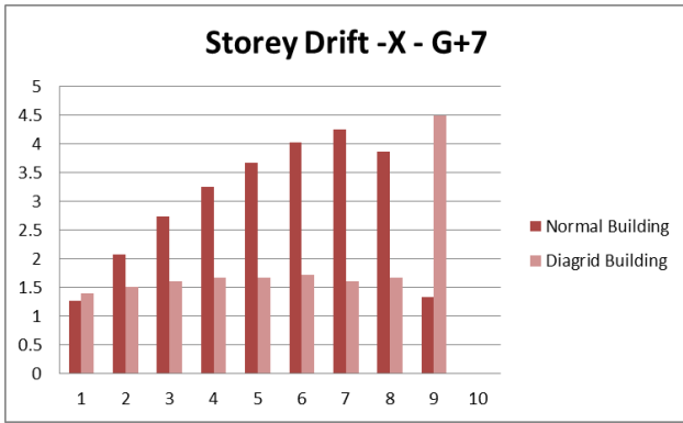
storey drift X for G + 7
