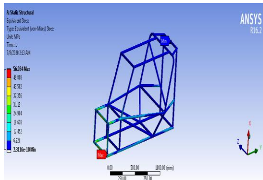
FIGURE 8VON-MISSES STRESS OF AISI 4130 MATERIAL
