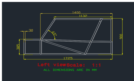
FIGURE 4 SIDE VIEW OF THE FRAME
