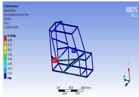
FIGURE 15 VON-MISES STRESS OF AISI 1018 MATERIAL
