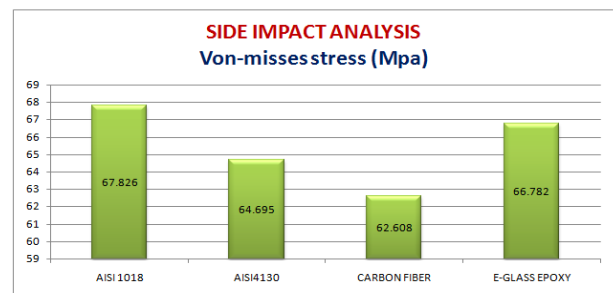
FIGURE 23 VONMISSES STRESS OF SIDE IMPACT
