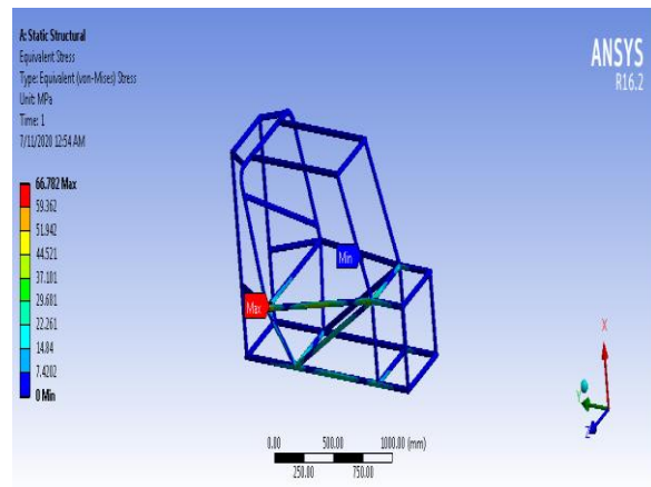
FIGURE 16 VON-MISES STRESS OF AISI 4130 MATERIAL
