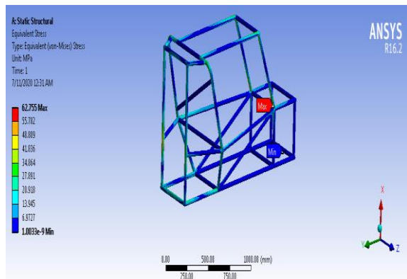
FIGURE 12 VON-MISES STRESS OF AISI 4130 MATERIAL
