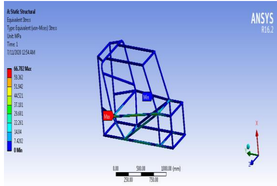
FIGURE 18 VON-MISSES STRESS OF E-GLASS FIBER MATERIAL
