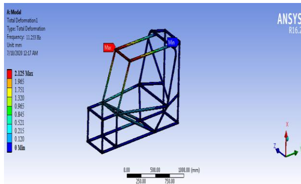
FIGURE 19 MODE 1 OF AISI 4130 MATERIAL
