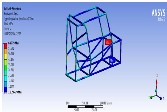
FIGURE 14 VON-MISES STRESS OF E-GLASS FIBER MATERIAL
