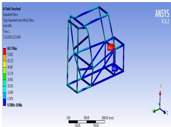
FIGURE 13 VON-MISES STRESS OF CARBON FIBER MATERIAL
