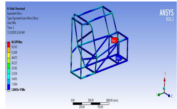
FIGURE 11 VON-MISSES STRESS OF AISI 1018 MATERIAL
