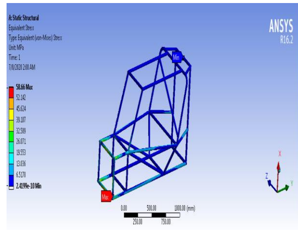
FIGURE 10 VON-MISSES STRESS OF E-GLASS FIBER MATERIAL
