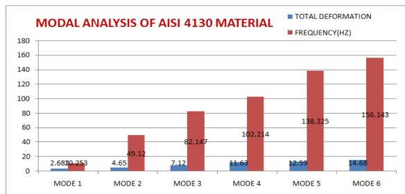
FIGURE 24 MODAL ANALYSIS OF AISI 4130 MATERIAL
