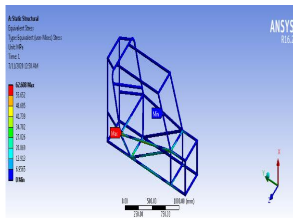
FIGURE 17 VON-MISES STRESS OF CARBON FIBER MATERIAL
