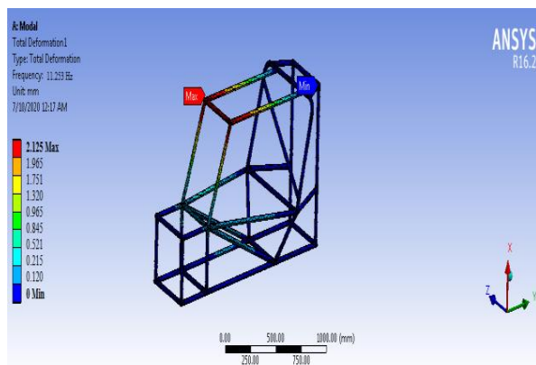
FIGURE 20 MODE 1 OF CARBON FIBER MATERIAL
