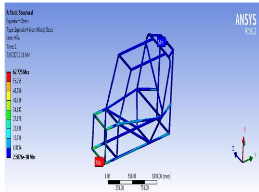
FIGURE 7 VON-MISSES STRESS OF AISI 1018 MATERIAL
