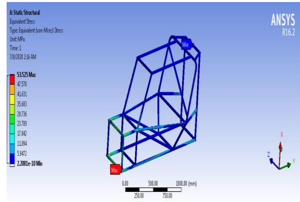
FIGURE 9 VON-MISSES STRESS OF CARBON FIBER MATERIAL
