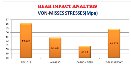
FIGURE 22 VONMISSES STRESS OF REAR IMPACT
