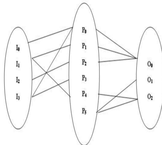
Figure. 2 Venn diagram
