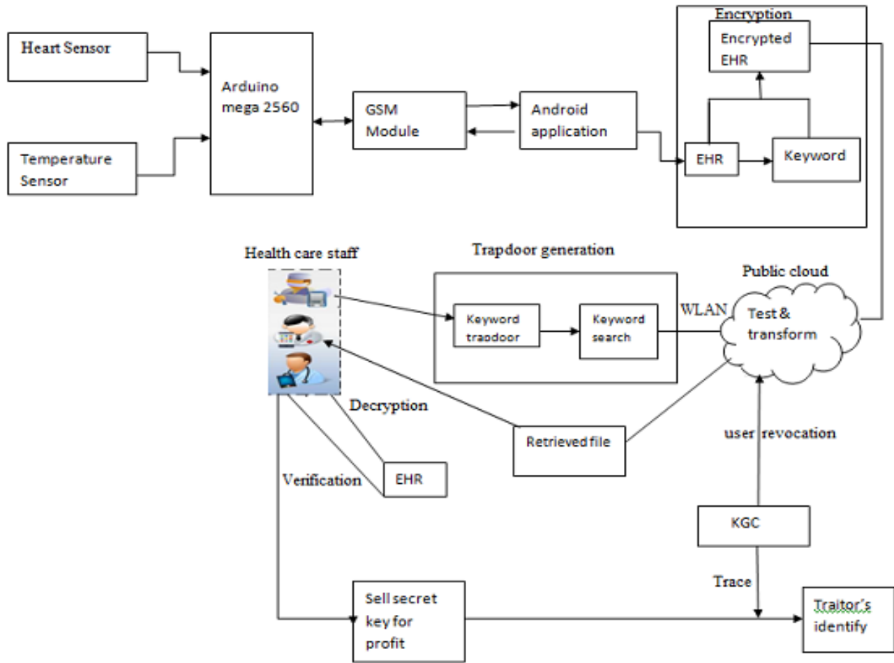
Figure 1. System Architecture
