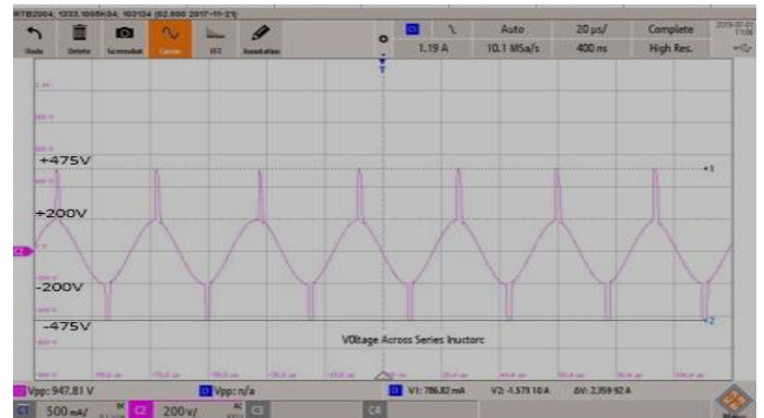
Fig. 7 Voltage across Series Inductor
