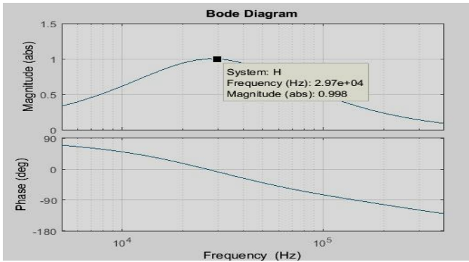
Fig. 4 Switching frequency and the gain is approximately unity
