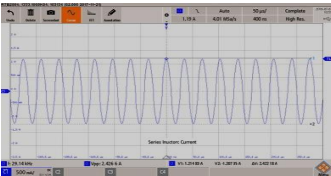
Fig. 9 Series Inductor L_s current
