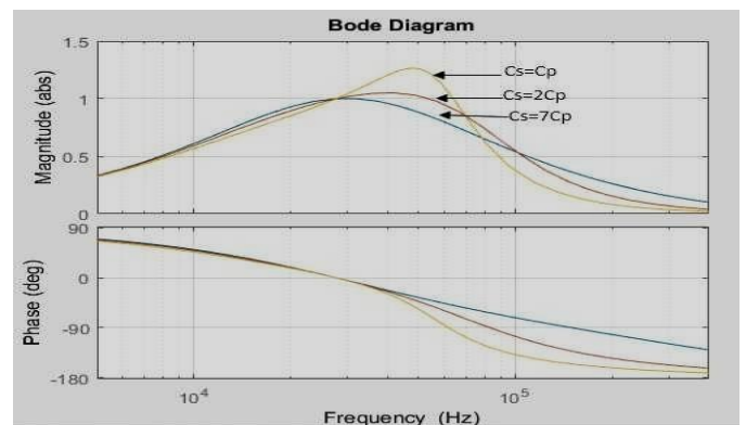
Fig. 3 The gain plot for different value of parallel capacitor
