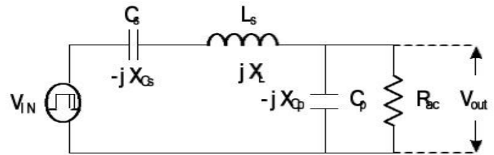
Fig. 2 Frequency domain circuit of the resonance tank
