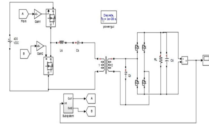
Fig. 1 LCC resonant converter circuit in MATLAB
