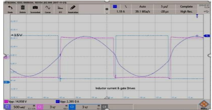
Fig. 6 Inductor current & Gate Drive
