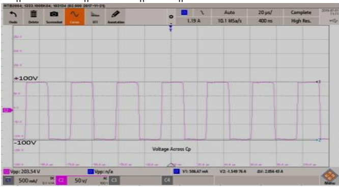
Fig. 8 Volate across transformer Primary side
