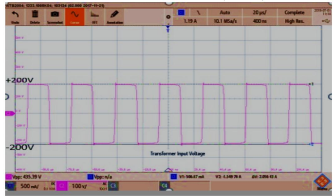
Fig. 5 Transformer Primary side voltage
